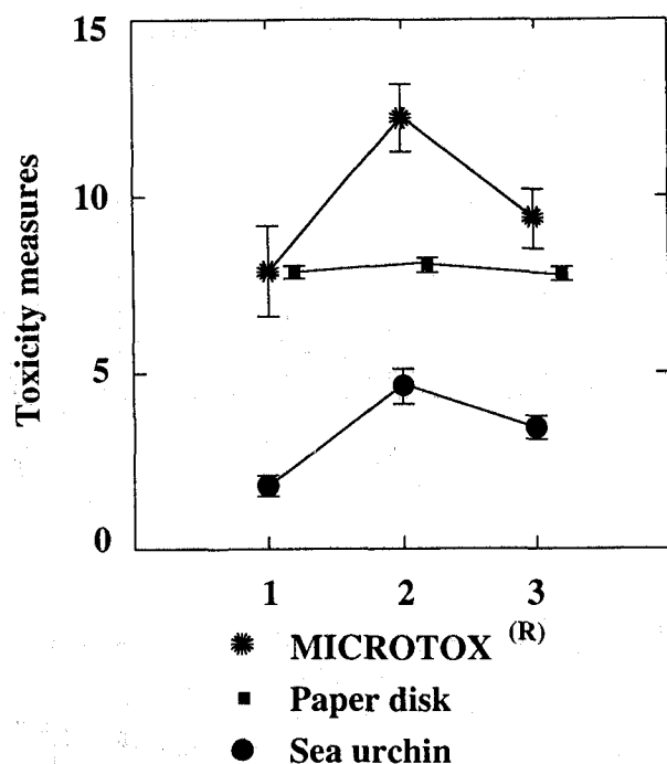
Figure 1. Toxicity measures obtained by the three methods for the size classes considered. Toxicity units in the ordinate differ in each test (TU, mm, and ppm for the MICROTOX®, paper disk, and sea urchin assays, respectively). Therefore, only the pattern of relative variation among size classes, not the absolute values, are comparable. Bars are standard errors.
